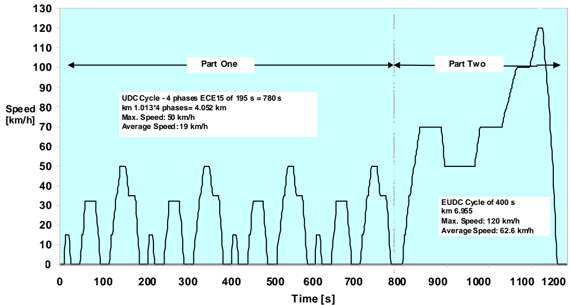
Figure 3.1 NEDC Cycle
