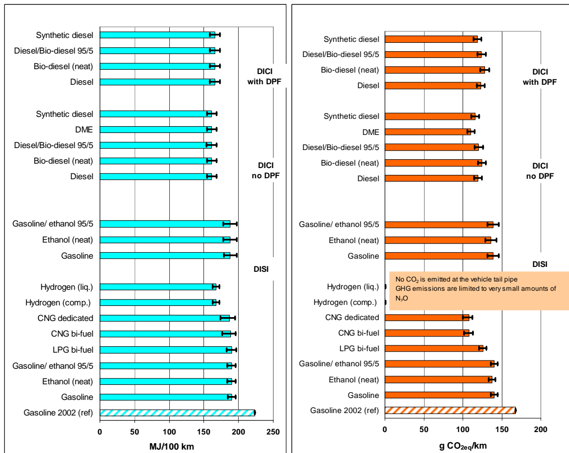
Figure 5.1.5a/b Average energy/fuel consumption and GHG emissions over the NEDC 2010+ ICE vehicles
